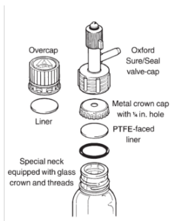
Fig. 1A Sure/Seal components
