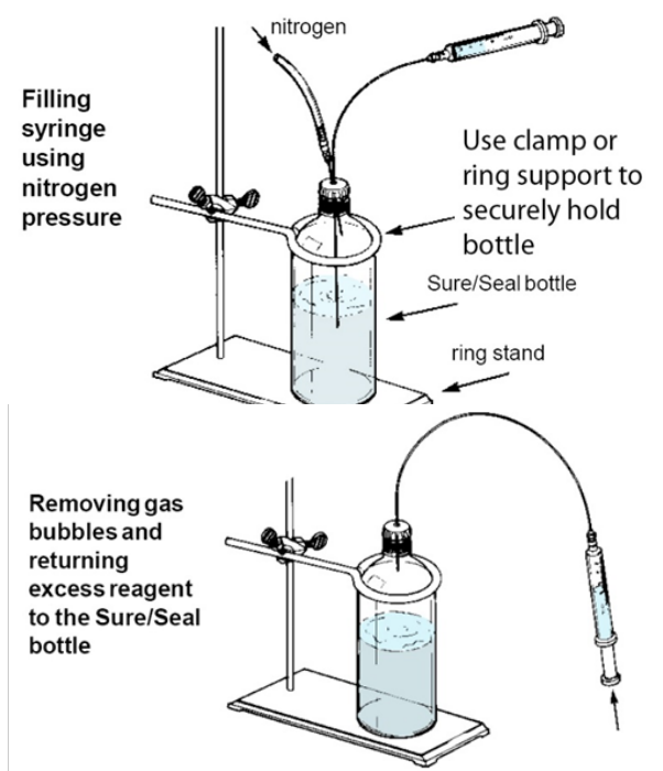
Fig. 2B. Removing gas bubbles and returning excess reagent to the Sure/Seal bottle
