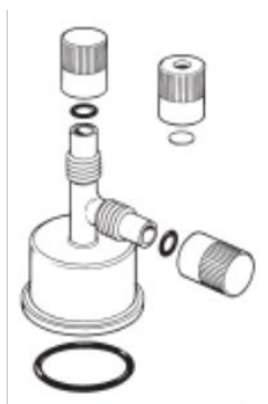
Fig. 1B. Sure/Seal septum-inlet transfer adapter
