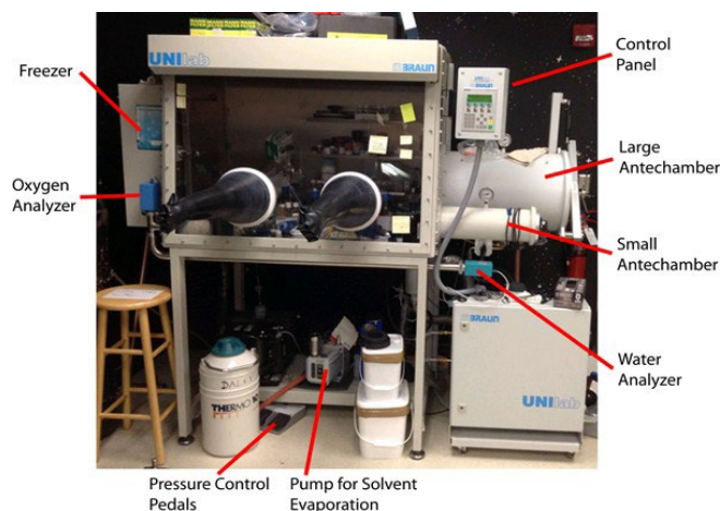
Figure 4.3 – Glovebox
