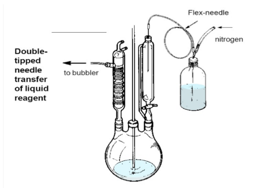
Fig. 3A. Double-tipped needle transfer of liquid reagent
