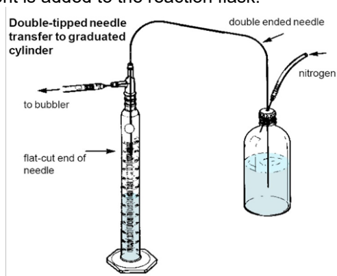
Fig. 3B. Double-tipped needle transfer to graduated cylinder
